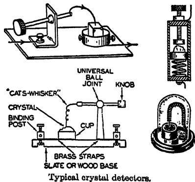
Typical crystal detectors.
